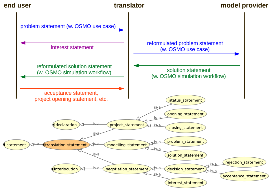
Fig. 1. Top: A possible interchange between participants of a materials modelling marketplace during steps 1 to 4 of a translation process, cf. Tab. 4, expressed in terms of mmtto:translation_statement entities. Bottom: Diagram showing the transitive reduction of the rdfs:subClassOf relation (grey arrows) for the mmtto:translation_statement branch of the MMTO, wherein evmpo:declaration , evmpo:interlocution , and evmpo:statement are entities from the European Virtual Marketplace Ontology (EVMPO) [22]; this diagram was generated using OWLViz [20].
